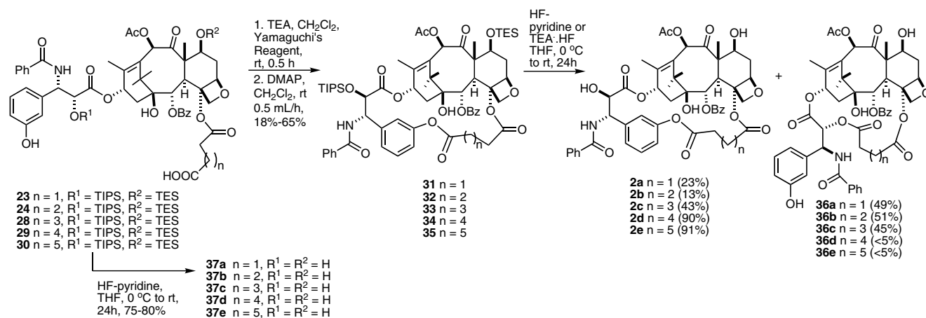
Scheme 6. Syntheses of the macrocyclic paclitaxel lactones.
