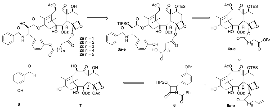
Scheme 1. Retrosynthetic analysis of macrocyclic paclitaxel lactone.
